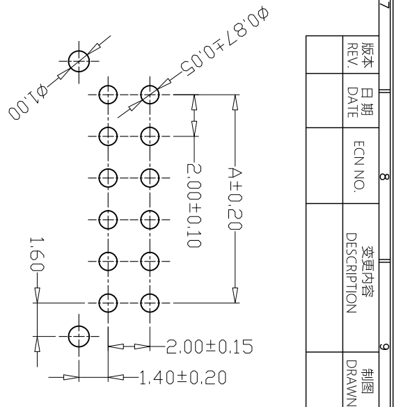
PCB LAYOUT
